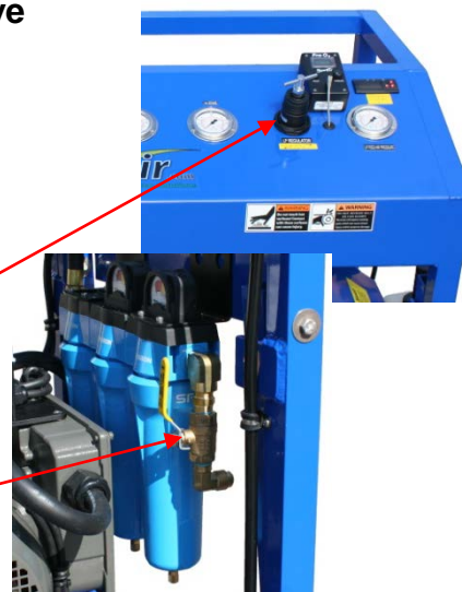
LP Supply Option Shown
