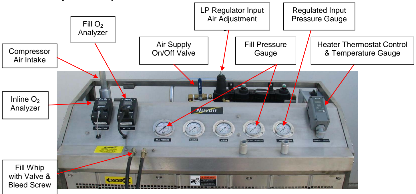
Front View – LP Supply Option Shown
