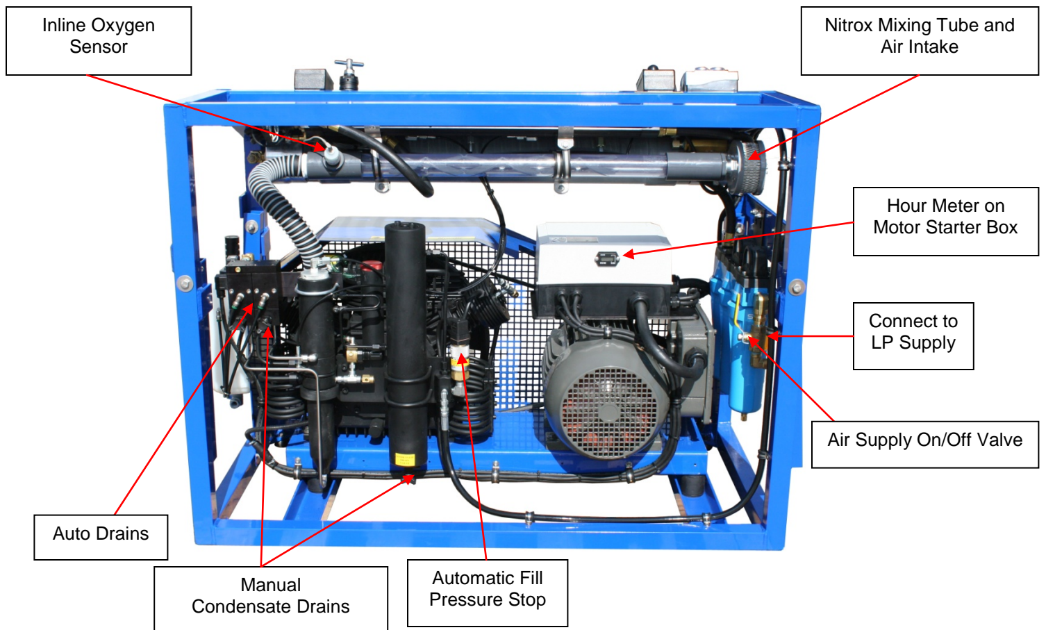
Rear View – LP Supply Option Shown
