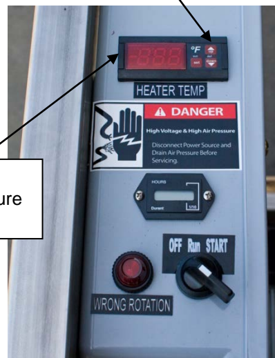
Heater Thermostat Control
