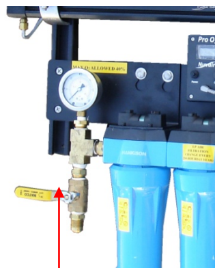
On/Off Air Flow Ball Valve Pictured in off position
