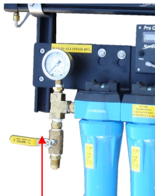
On/Off Air Flow Ball Valve Pictured in off position
