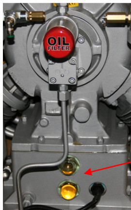
Compressor Lubricant Level Sight Gauges
